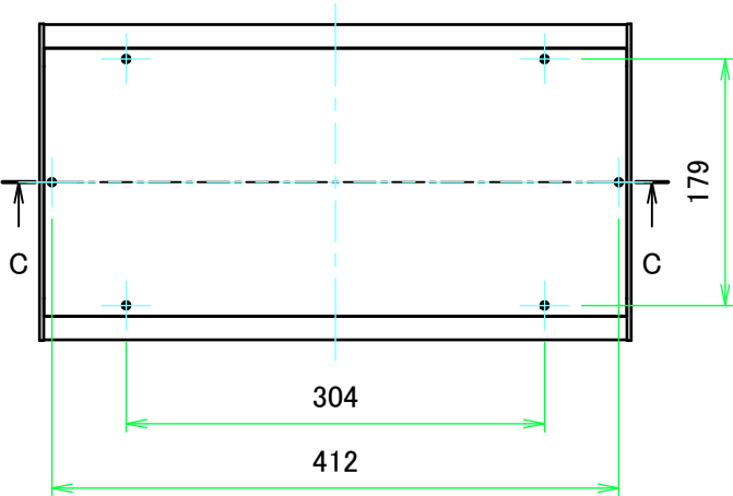
E view
